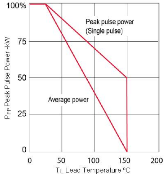
FIGURE 3 Derating Curve
